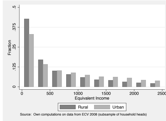
Figure 4.5: Equivalent income measures
