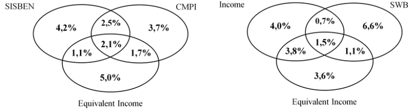
Figure 4.6: Overlap between the individuals identified as worst-off
