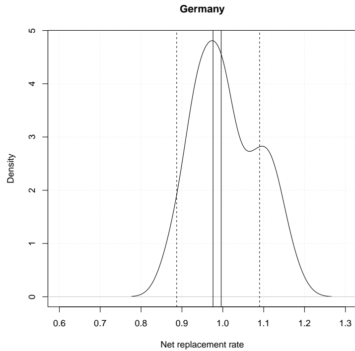
Figure 1: Kernel density estimates of the net replacement rates resulting from different welfare indicators, income concepts, and definitions of the retirement status. For the US results are based on 157 estimates of net replacement rates; for Germany on 58 estimates. Source: Own calculations using HRS and EVS.
